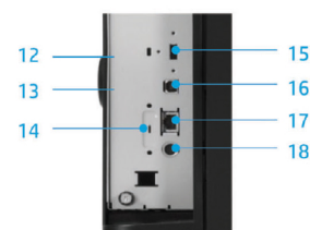
Close-up of I/O ports
